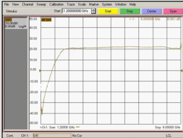
(Fig 1) TS-6842A Gain Versus Frequency
